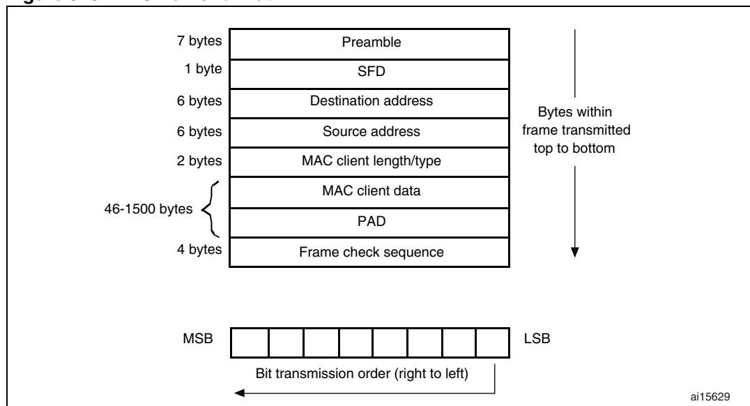
Figure 316. MAC frame format
