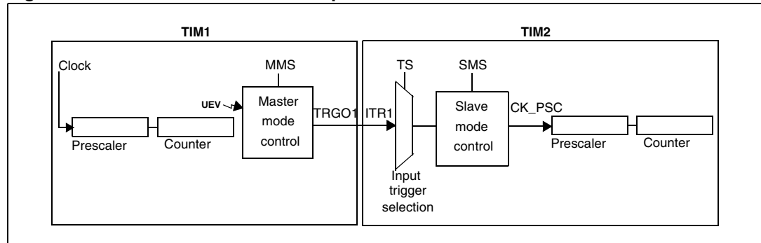
Figure 152. Master/Slave timer example
